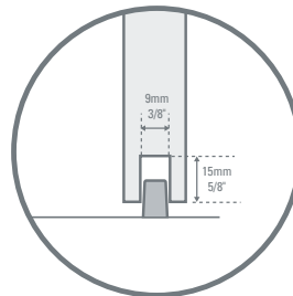
GUIDE INSTALLATION
