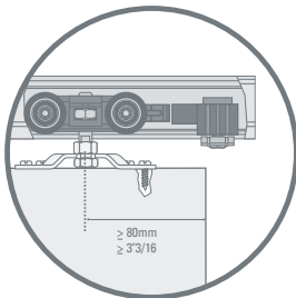
CARRIER INSTALLATION
