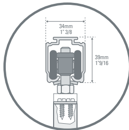
TRACK INSTALLATION
